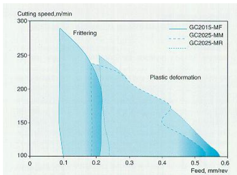
Figure 1. Machining chart for Sanmac 4571.
