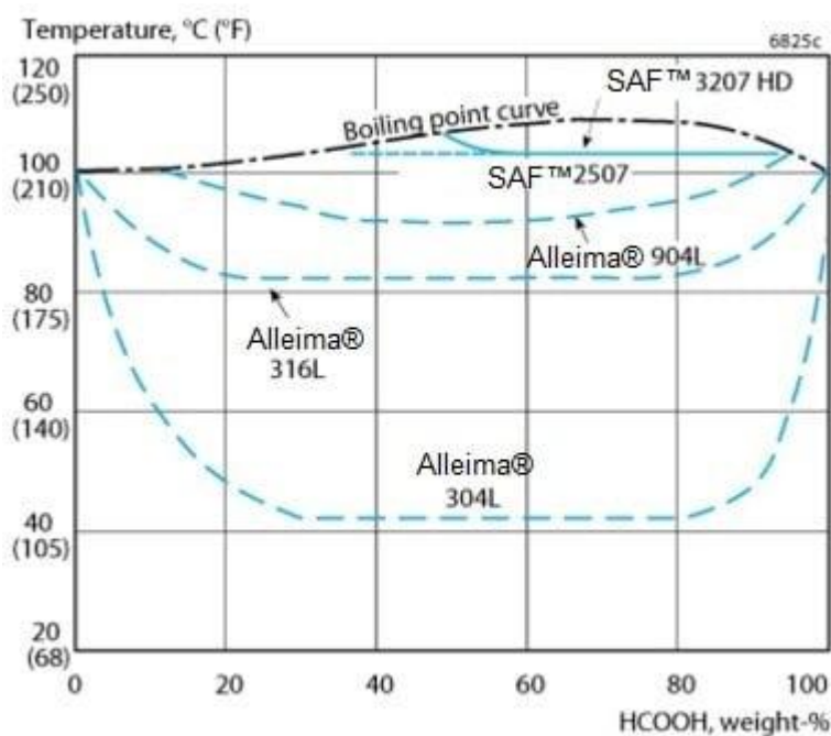
Figure 1. Isocorrosion diagram in formic acid. The curves represent a corrosion rate of 0.1 mm/year (4 mpy) in a stagnant test solution.
