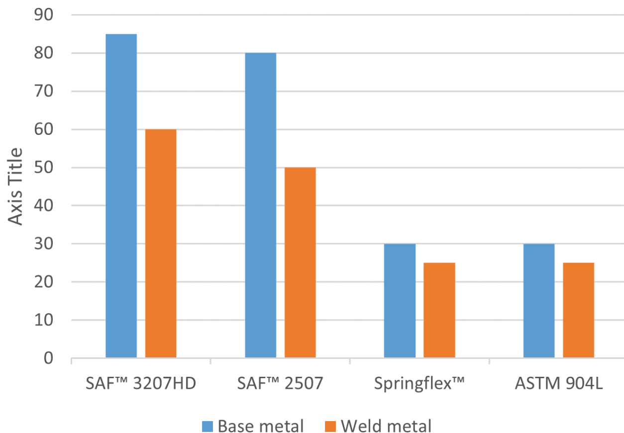
Figure 4. Critical pitting corrosion temperature (CPT) of base material and weld metal of three duplex grades and one austenitic grade.
