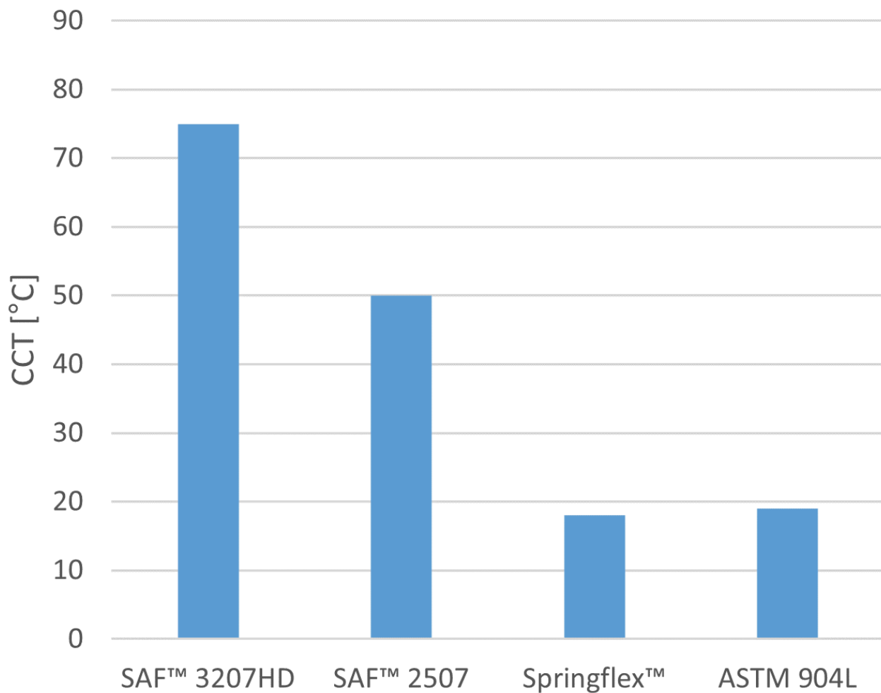
Figure 5. Critical crevice corrosion temperature (CCT) of three duplex grades and one austenitic grade.
