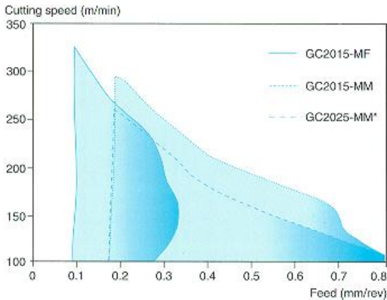
Figure 1. Machining chart for Sanmac® 316/316L.
