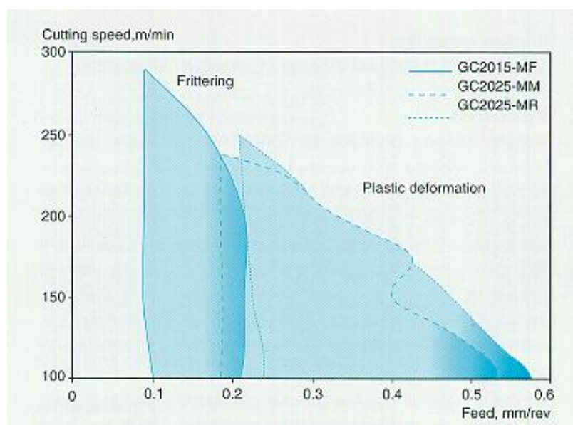
Figure 1. Machining chart for Sanmac 4571.
